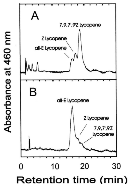
Fig. 1. HPLC separation of carotenoids from E. coli pACCRT-EBP/pBBR1MCS2zds/pTrc99A (A) and E. coli pACCRT-EBP/pBBR1MCS2zds/pTrc-0033 (B). Separation was carried out on a Nucleosil C 18 3 \mu column with acetonitrile/methanol/2-propanol (85:10:5).
