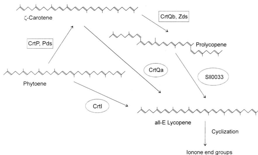
Fig. 2. Reaction sequences from phytoene to all- E lycopene involving different gene products. CrtI, 4-step phytoene desaturase from bacteria or archaeobacteria; CrtP and Pds, 2-step phytoene desaturases from cyanobacteria and plants; CrtQb and Zds, \zeta -carotene desaturase from cyanobacterial and plants; CrtQa, \zeta -carotene desaturase from Anabaena 7120; Sll0033 carotene isomerase from Synechocystis 6803. Boxes and circles indicate the structural relationship to the pds - or crtI -type of carotene desaturases, respectively.
